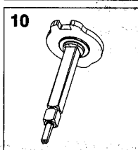
10 Drive Hub & Spindle Assembly 118-507721-2 FOR DOOR THICKNESS FROM 1.75" (45mm) TO 2.00" (51mm) 118-507721-3 FOR DOOR THICKNESS FROM 2.25" (57mm) TO 2.50" (64mm)
