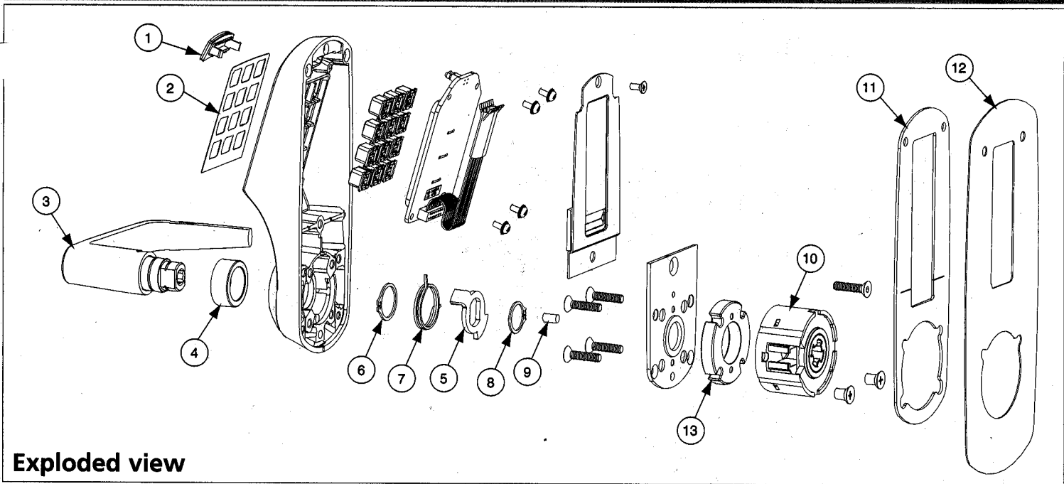
1 Cosmetic Window Sub Assembly 118-507725
