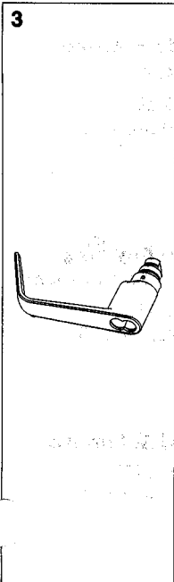
3 Outside Lever Sub Assembly 118-507718 *Best 5, 6, 7 pins 118-508717-L *LH Yale 7 pins 118-508717-R *RH Yale 7 pins 118-508716-L *LH Yale 6 pins 118-508716-R *RH Yale 6 pins 118-508712-L *LH Assa 6 pins Medeco 5 & 6 pins 118-508712-R *RH Assa 6 pins Medeco 5 & 6 pins 118-508710 *Schlage 118-509086-L *LH Ilco 7 pins 118-509086-R *RH Ilco 7 pins
